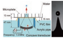
Ejection of micro droplet with focused ultrasound
