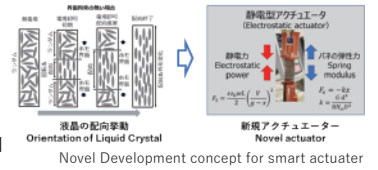
Novel Development concept for smart actuator
