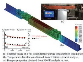
Full-scale viscoelastic damper experiment and simulation (stiffness, damping, temperature)
