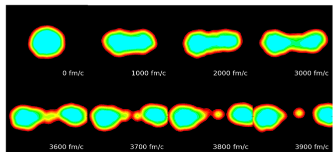
Simulation of ^{256}\text{No} fission using a microscopic reaction model
